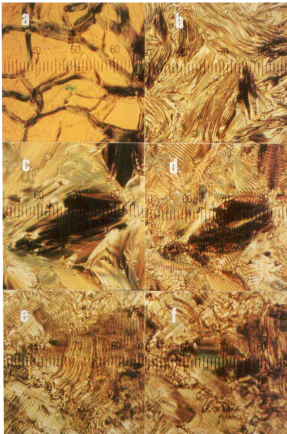
Figure 1. Typical polarizing optical microscopic textures of the mesophases of compound D8. (a) Cholesteric oily-streak texture ( T = 129.5^\circ\text{C} ), (b) texture of the twist grain boundary or TGB A^* phase ( T = 129.3^\circ\text{C} ), (c) fan-shaped texture of the chiral smectic A ( S_A^* ) phase ( T = 128.9^\circ\text{C} ), (d) fan-shaped texture with disclination lines of the S_C^* phase ( T = 125.6^\circ\text{C} ), (e) S_I^* texture with disclination lines ( T = 92^\circ\text{C} ) and (f) texture of the S_F^* phase. The sample was prepared on a glass slide with a cover slip without surface alignment layers. (10 units of scale \triangleq 60\ \mu\text{m} .)
