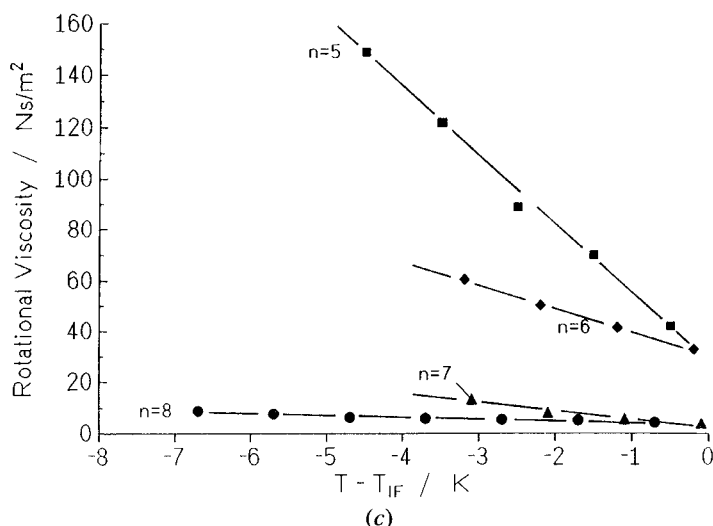
Figure 8. Temperature dependence of the effective rotational viscosity \gamma_\phi for the compounds D5–D8 in the (a) S_C^* , (b) S_I^* and (c) S_F^* phases. The effective rotational viscosities increase with decreasing length of the alkyl chain at all three ferroelectric phases.
